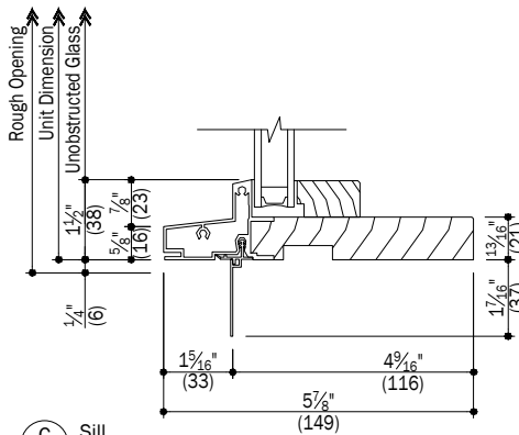
C Sill AKR - Complementary to 400 Series Tilt-Wash, Woodwright, FW Hinged, FW Gliding 200 Series Inswing Patio Door, Narroline, Permashield
