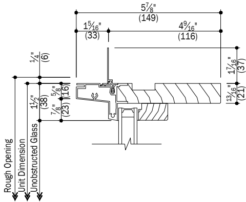
A Head AKR - Complementary to 400 Series Tilt-Wash, Woodwright, FW Hinged, FW Gliding 200 Series Inswing Patio Door, Narroline, Permashield
