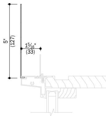
F 5" Aluminum Clad Frame Expander
