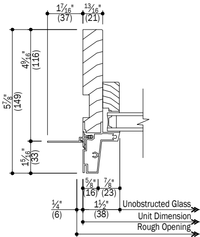
B Jamb AKR - Complementary to 400 Series Tilt-Wash, Woodwright, FW Hinged, FW Gliding 200 Series Inswing Patio Door, Narroline, Permashield
