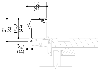
D 2" Aluminum Clad Brickmould
