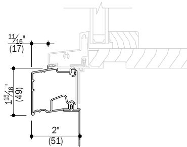
E Aluminum Clad Sillnose
