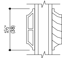
P 6 1 1/2" Simulated Divided Light
