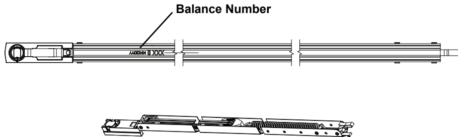
Tilt-Wash Insert Sash Balancer
