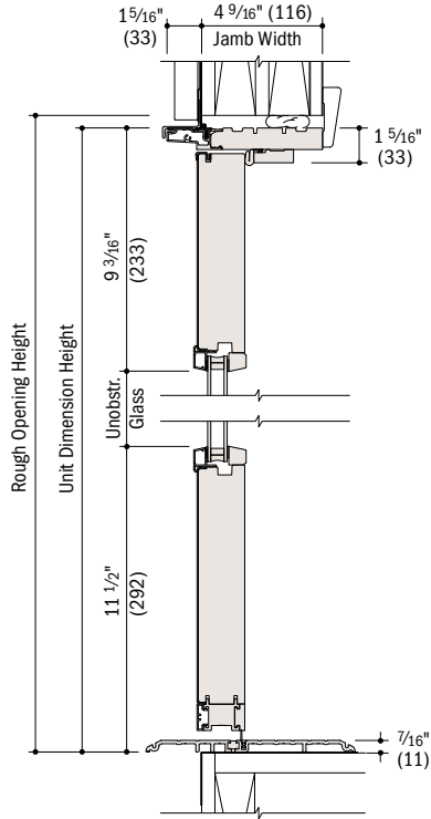
Vertical Section
