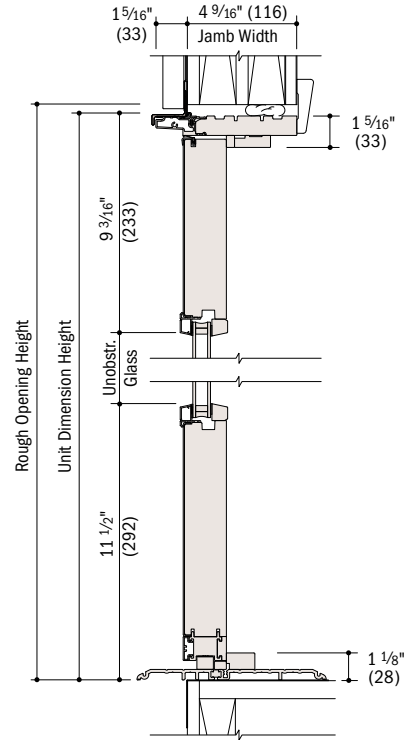
Vertical Section
