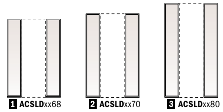
Direct-set (ACSLD) commercial outswing entry door sidelights.
